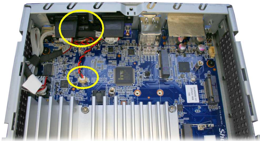
Photo: Position of the button cell battery and the connector on the mainboard with the computer housing open.
